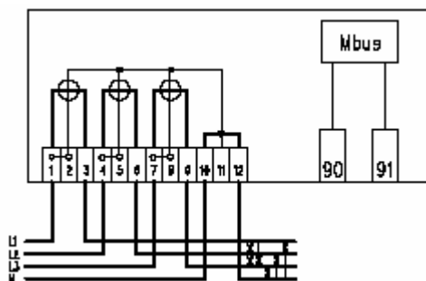
Fig. 46: Connection diagram of MT371 meter with M-Bus communication interface
