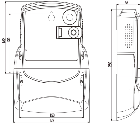
Fig. 15a: Overall and fixing dimensions of an MT371 meter fitted with a long terminal cover
