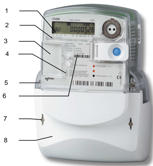
Fig. 9: MT372 meter constituent parts
