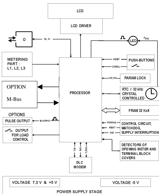
Fig. 19: MT371 meter block diagram
