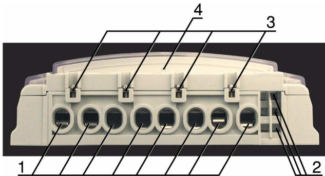
Fig. 10: A terminal block of MT371 meter – bottom view
