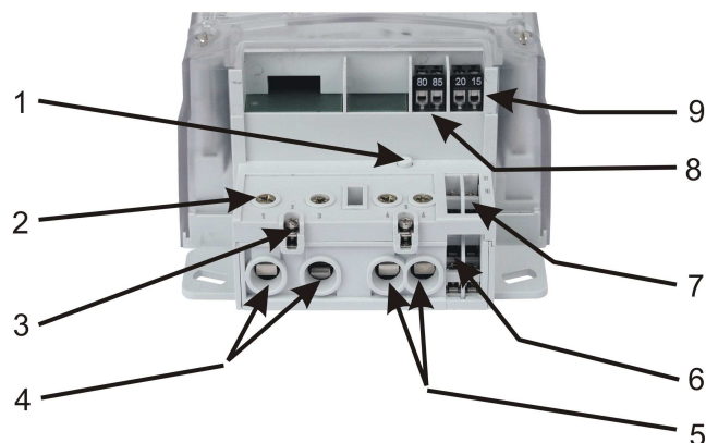
Fig. 4: A terminal block of ME37y meter
