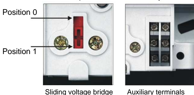
Fig. 12a: A terminal block – sliding voltage bridge and auxiliary terminals
