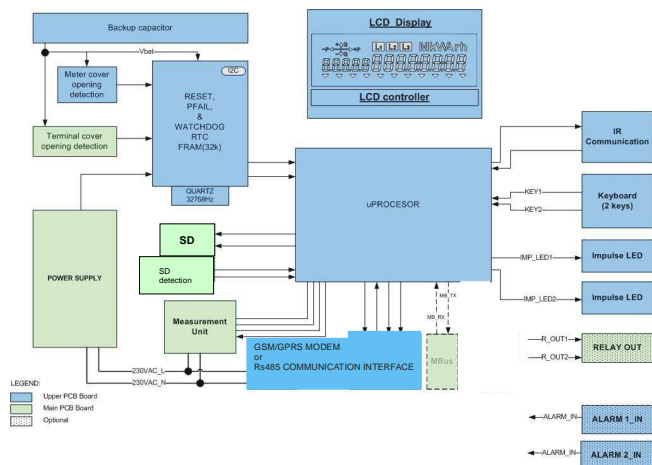
Fig. 7: ME372 meter block diagram
