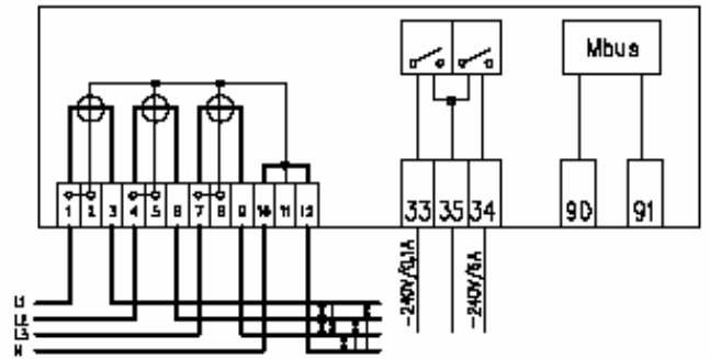
Fig. 47: Connection diagram of MT371 meter with outputs and M-Bus communication interface
