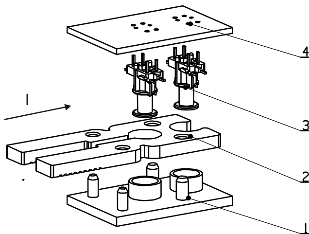
Fig. 22: Explosion view of the Rogowski coil
