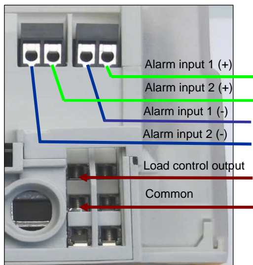
Fig. 32: Position of alarm inputs and outputs on ME37y meters – bottom view
