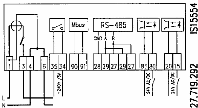
Fig. 44: Connection diagram of ME372 meter with RS 485 communication interface
