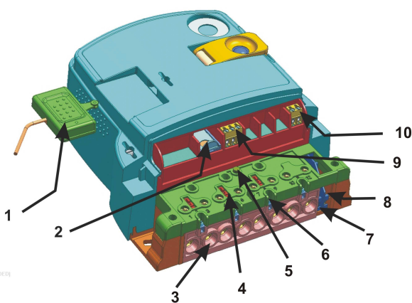
Fig. 13: Details of a terminal block for GSM/GPRS meter
