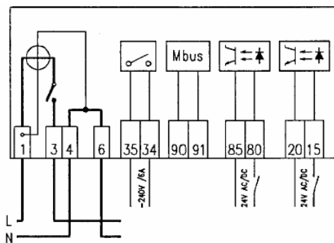
Fig. 43: Connection diagram of ME371 meter
