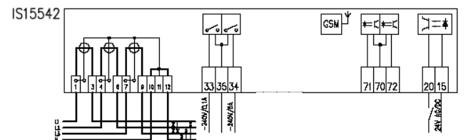
Fig. 49: Connection diagram of MT372 meter with GSM/GPRS modem
