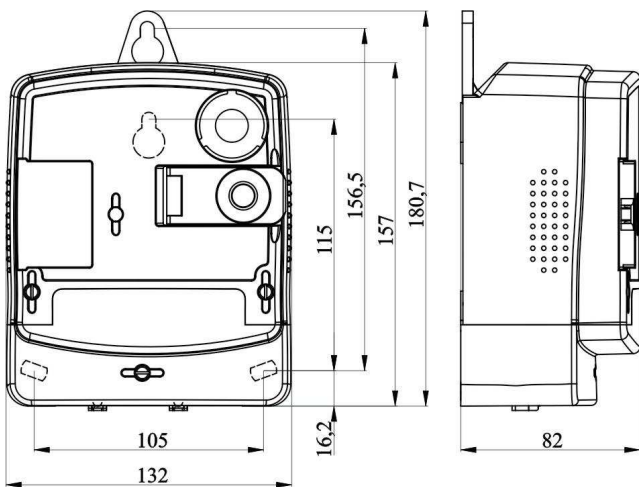
Fig. 5b: Overall and fixing dimensions of a meter fitted with a short terminal cover
