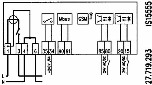
Fig. 45: Connection diagram of ME372 meter with GSM/GPRS modem
