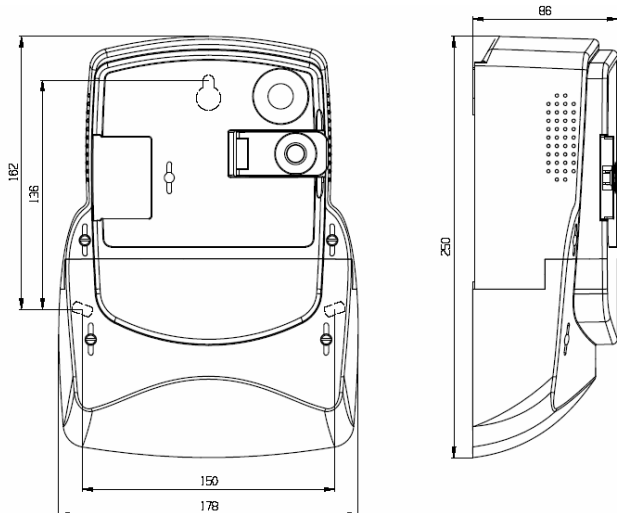
Fig. 17a: Overall and fixing dimensions of an MT372 meter fitted with a long terminal cover
