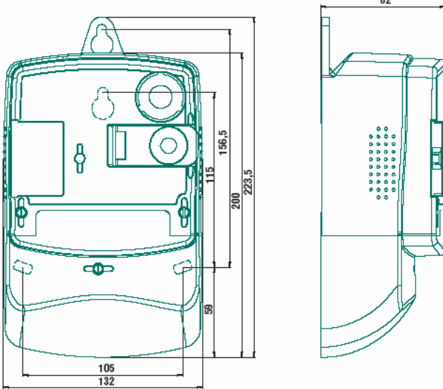
Fig. 5a: Overall and fixing dimensions of a meter fitted with a long terminal cover
