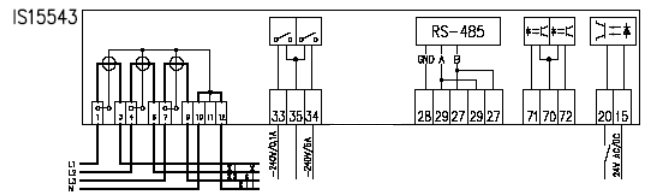
Fig. 48: Connection diagram of MT372 meter with RS 485 communication interface
