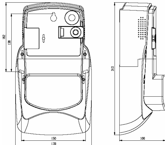
Fig. 18: Overall and fixing dimensions of an MT372 meter fitted with a switching device and a long terminal cover
