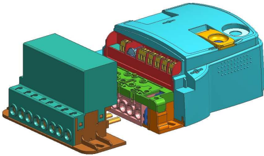
Fig. 34: Assembly of Z03 plug-in switching device
