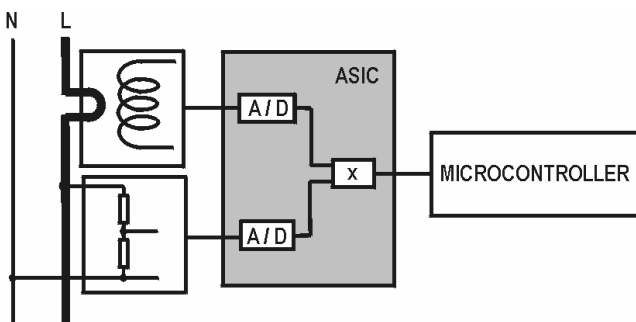
Fig. 21: Metering element
