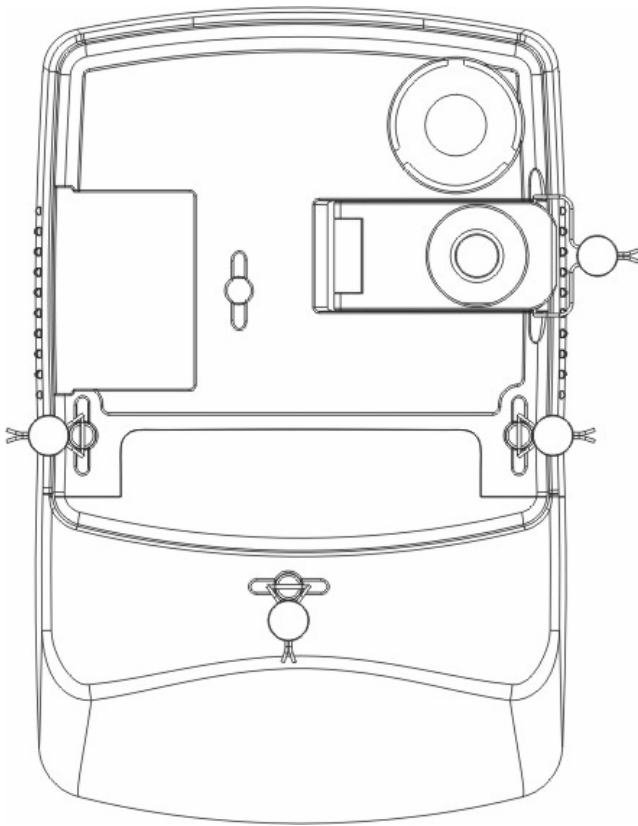
Fig. 37: ME37y meter position of the seals
