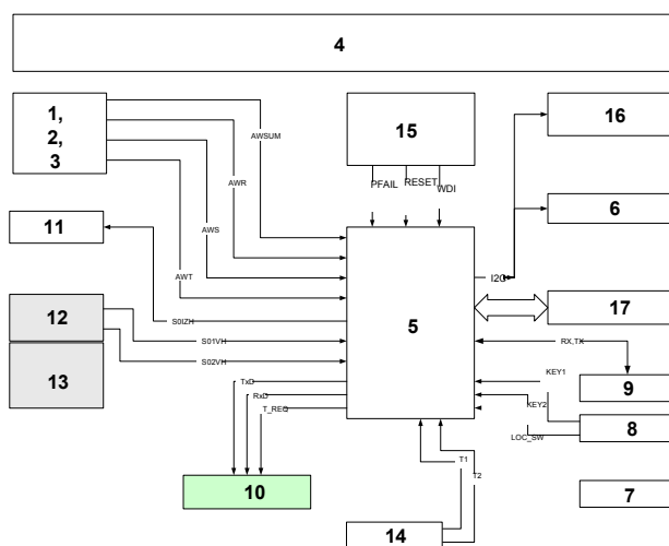
Fig. 20: MT372 meter block diagram
