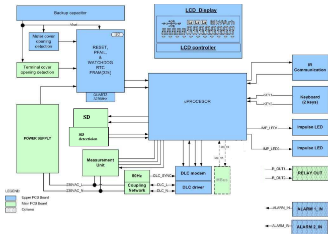
Fig. 6: ME371 meter block diagram
