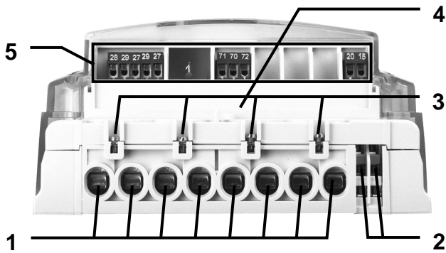
Fig. 11: A terminal block of MT372 meter – bottom view
